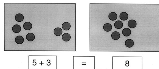
Figure 1. Representation of 5 + 3 = 8 .
