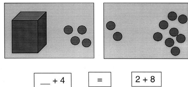
Figure 3. Concrete representation of \_ + 4 and 2 + 8 .
