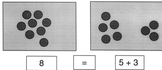
Figure 2. Concrete representation of 8 = 5 + 3 .
