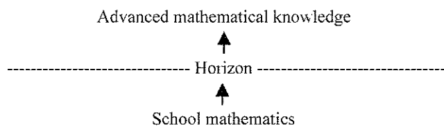
Figure 1. Knowledge at the mathematical horizon
