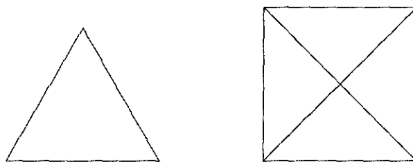
Figure 4 Simpler examples
